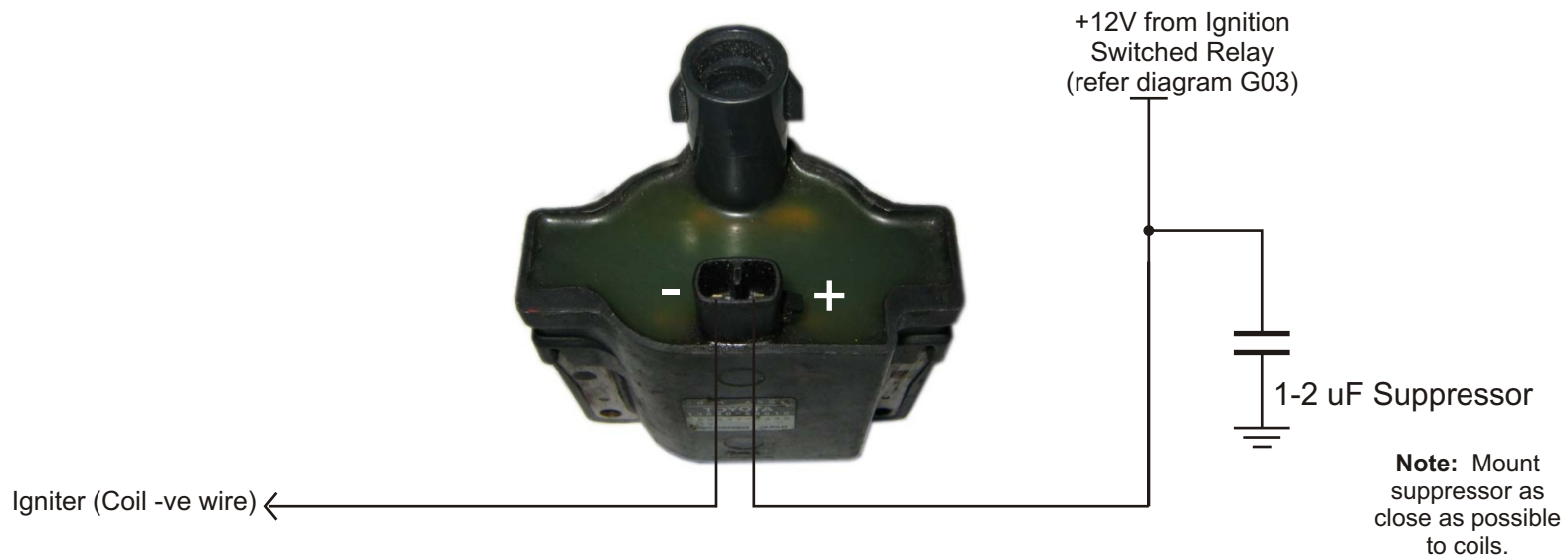
Figure 12.1 - Toyota 1UZFE Coil Wiring
