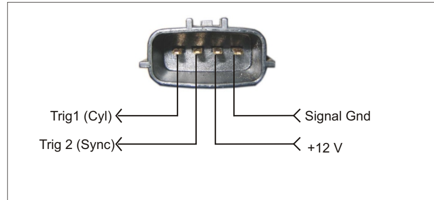
Figure C01.2 - Nissan ECCS CAS Pinout (non G3 ECU's)
