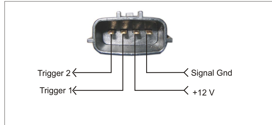
Figure C01.3 - Nissan ECCS CAS Pinout (G3 ECU's)
