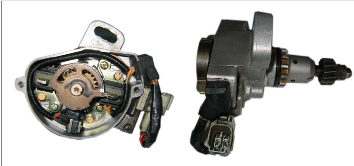
Figure C04.1 - Toyota 4AGZE Distributor/CAS
