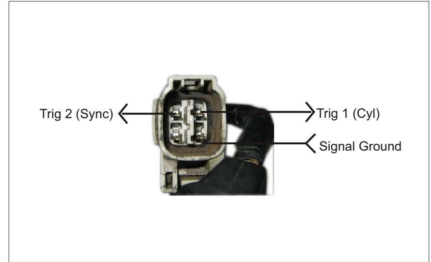
Figure C04.2 - Toyota 4AGZE Distributor/CAS Pinout
