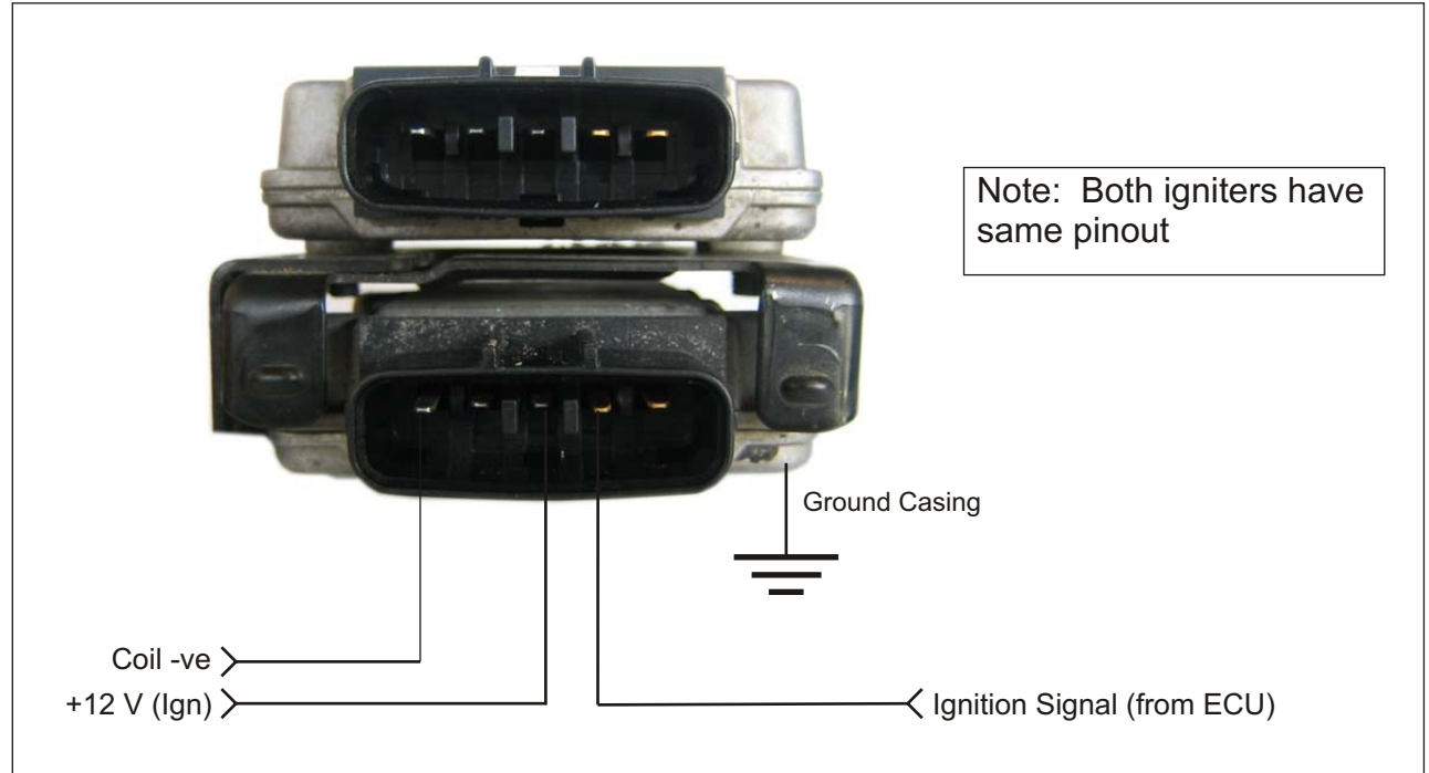
Figure I08.2 - Toyota 1UZFE Igniter Pinout
