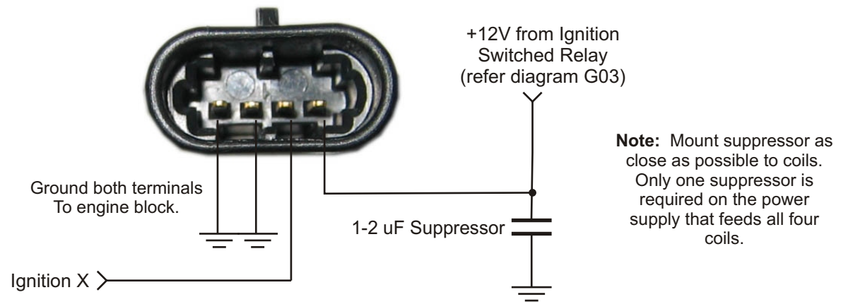
Figure I16.2 - LS 2/LS 7 Internal Ignitor Coil Wiring
