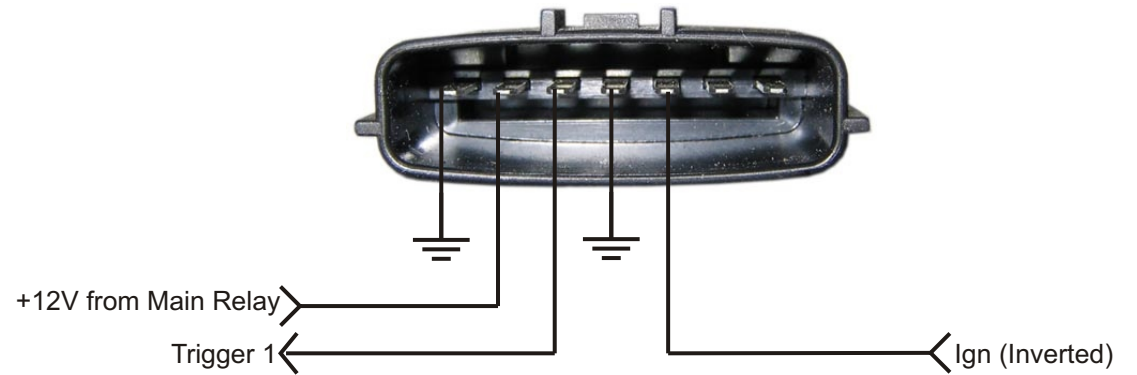
Figure C15.2 - Honda EX Civic 1600 Crank Angle Sensor Wiring
