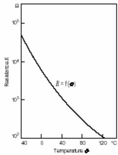
Temperature-sensor characteristic curve.
